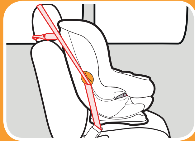
Vehicle Lap/Shoulder Seat Belt
